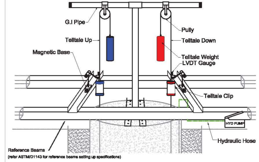
Telltale Pipe Measuring System
