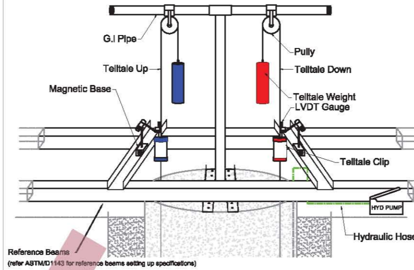
Telltale Wires Measuring System
